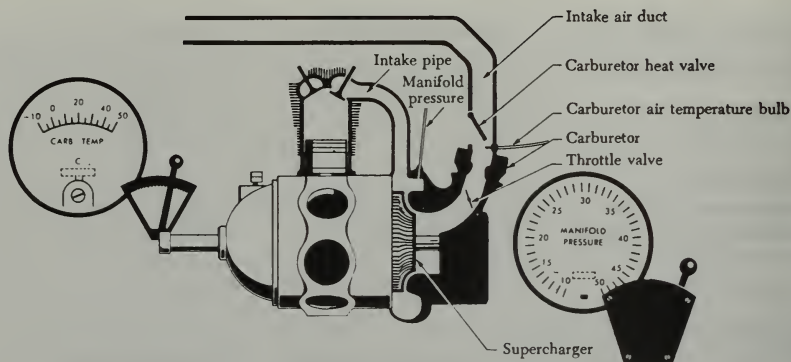
FIGURE 2-3. Simple induction system.
